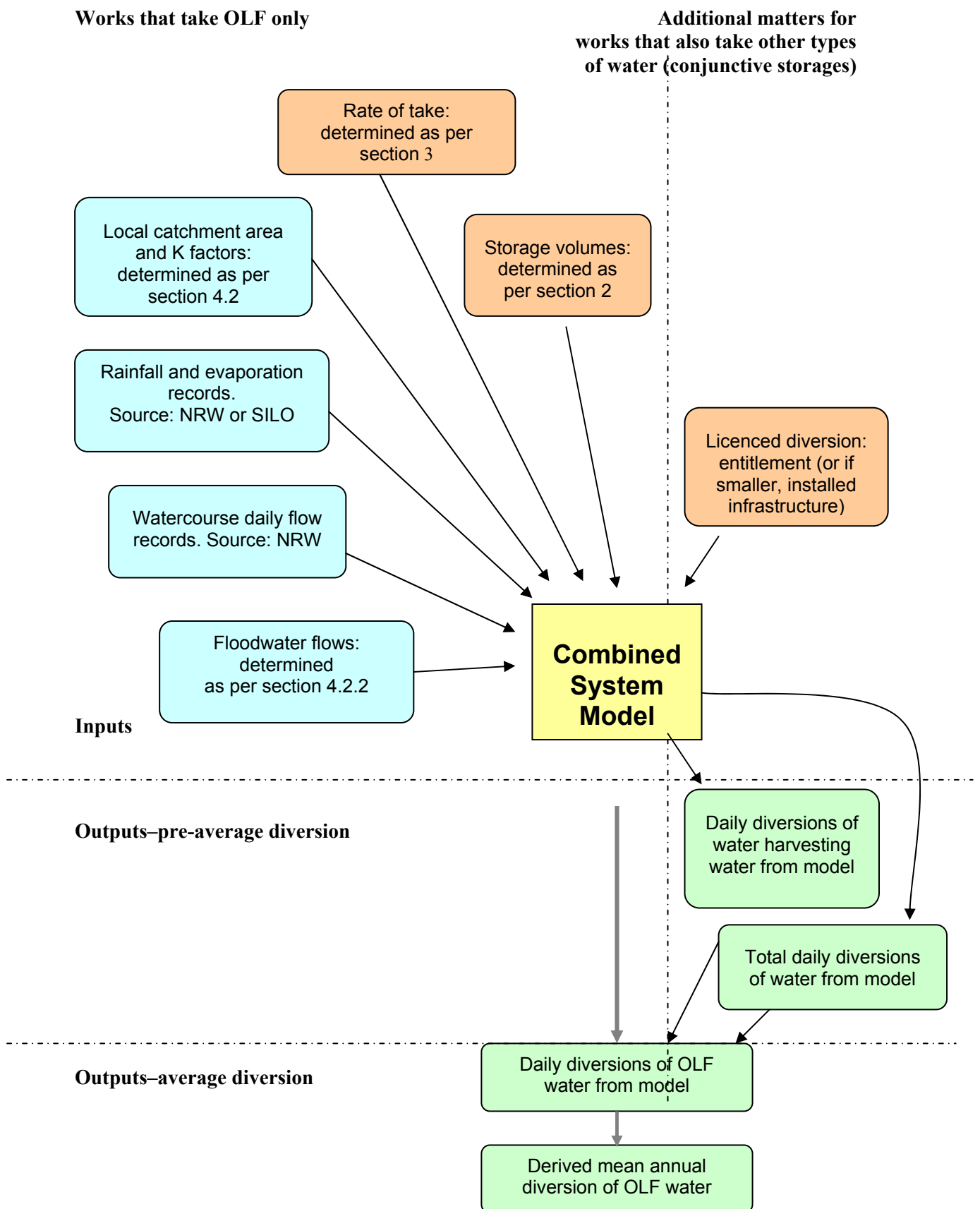
Figure 5: Modelling average annual diversion–overland flow take
